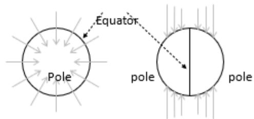
Positron's nuclear field Figure 12.14
