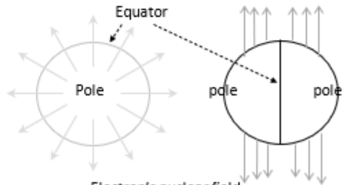
Electron's nuclear field Figure 12.19
