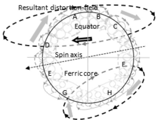
Resultant distortion-field Figure 17.22
