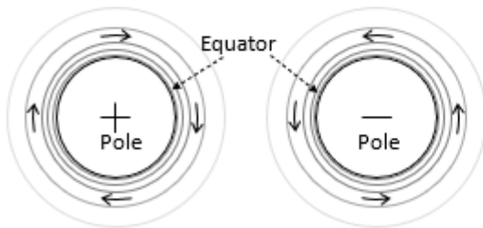
Electron's electric field Figure 12.18
