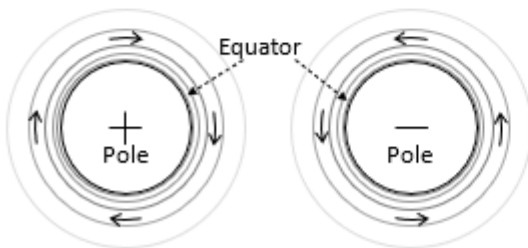
Positron's electric field Figure 12.13
