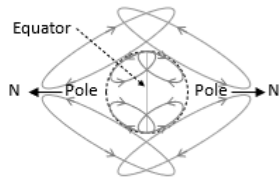
Positron's magnetic field Figure 12.12
