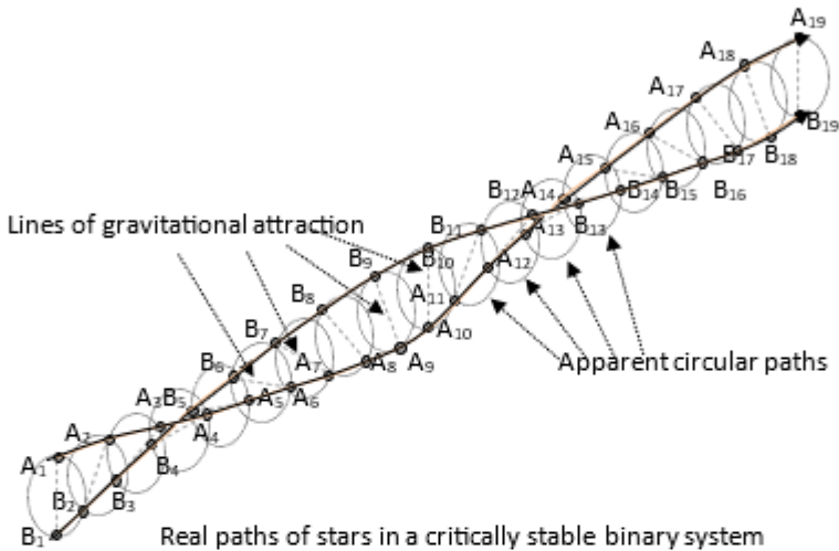
Real paths of stars in a critically stable binary system Figure 16.1.
