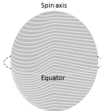
3D matter-core of photon Figure 4.2
