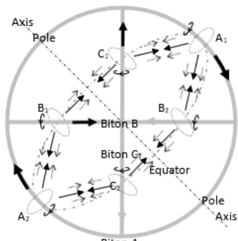
Biton A Figure 12.4
