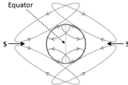
Electron's magnetic field Figure 12.17
